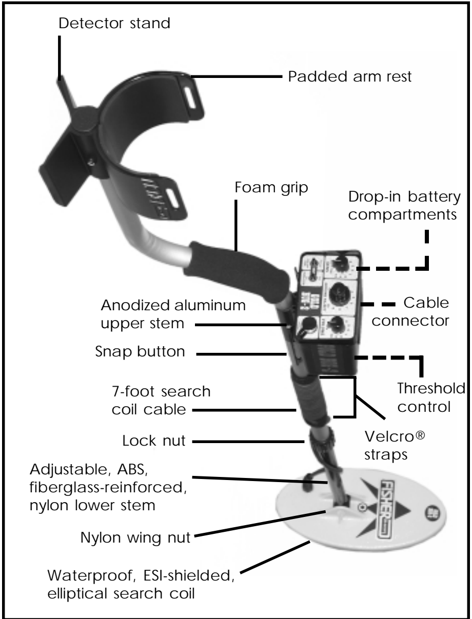
Figure 1. Fisher M-Scope Gold Bug
